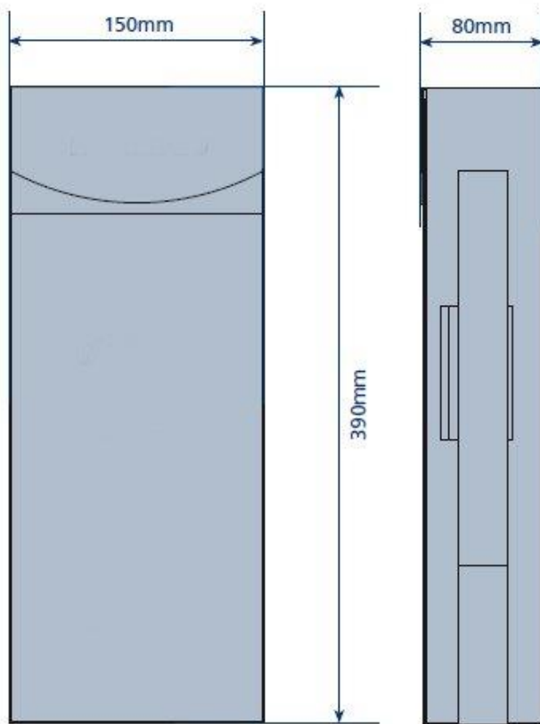
Storage case
